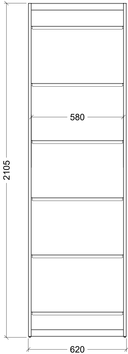
LJ013a - LJ Reverse shelving - base setup 1 frame + 6 shelves
